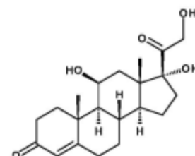
Hydrocortisone
