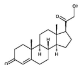
Deoxycorticosterone
