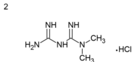
Metformin hydrochloride
