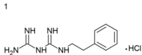
Phenformin hydrochloride
