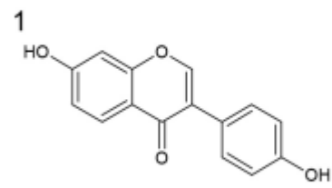
Daidzein
