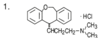
Doxepin hydrochloride
