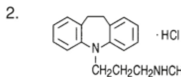
Desipramine hydrochloride
