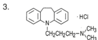
Imipramine hydrochloride
