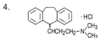
Amitriptyline hydrochloride
