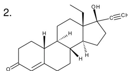
D-Norgestrel (Levonorgestrel)
